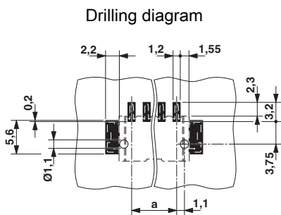
Type: PTSM 0,5/...-PL-2,5 ... with PTSM 0,5/...-HH-2,5-SMD... R...
