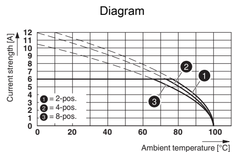
Type: PTSM 0,5/...-P-2,5 WH... with PTSM 0,5/...-HH0-2,5-SMD WH R...
